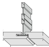
T section, long edge shiplap AW
